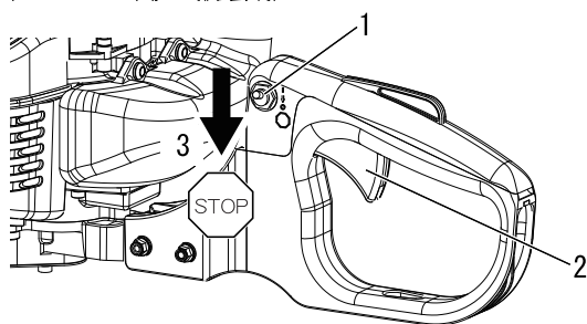
1. Ignition switch 2. Throttle trigger
