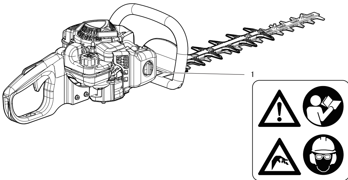
1. Safety decal (Part number X505-002030)
